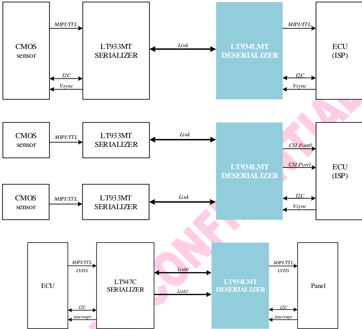
Figure 3.1 Application Diagrams
