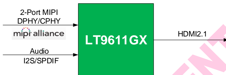
Figure 3.1 Application Diagram
