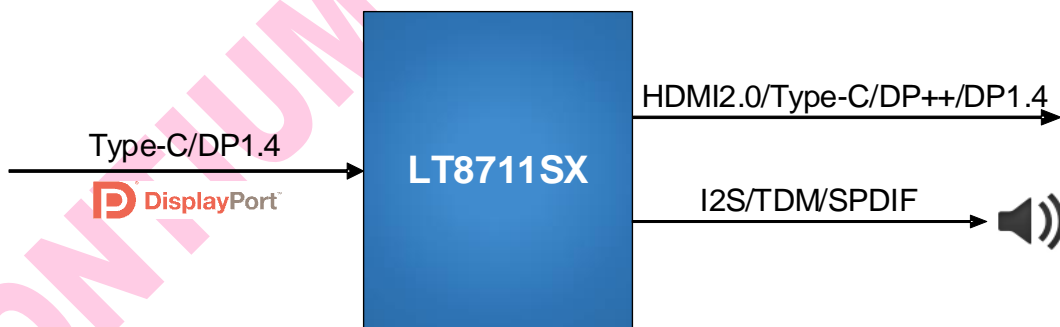
Figure 3.1. Application Diagram
