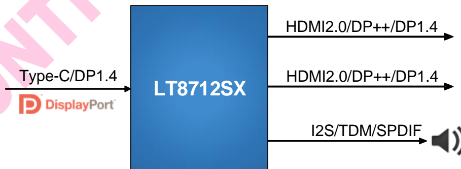
Figure 3.1. Application Diagram
