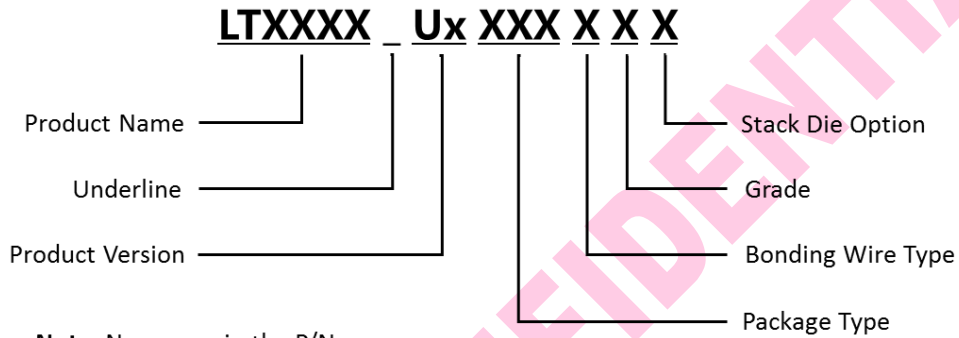
Figure 4.1 Part Number Naming Rules
